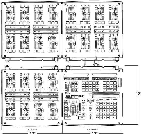
24/48 Manual Console
